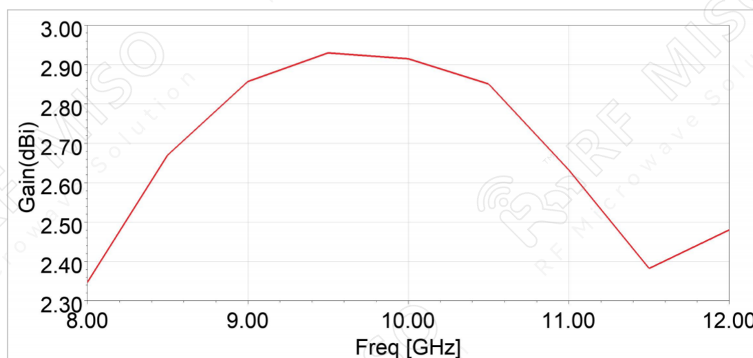
Gain
