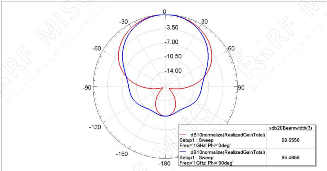
Gain Pattern
