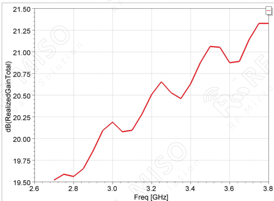
Gain
