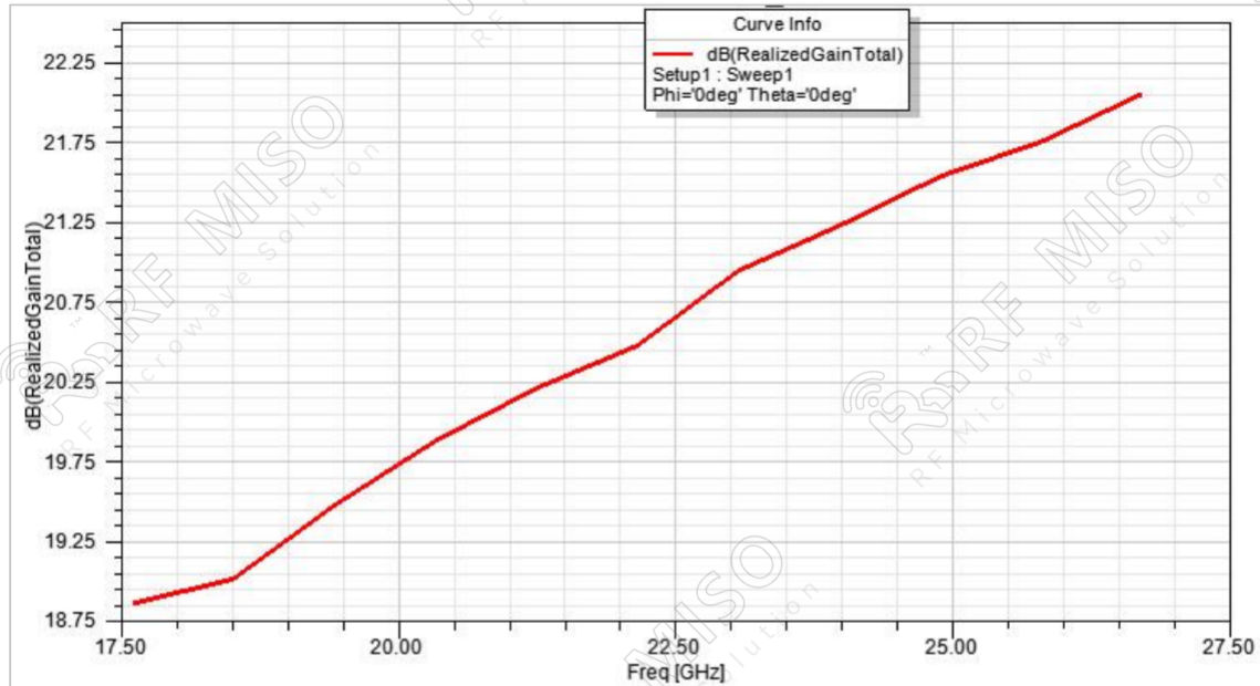
Gain
