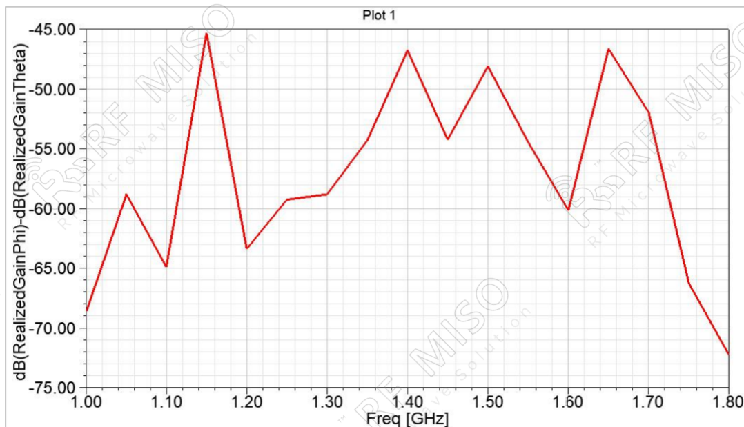
Polarization
